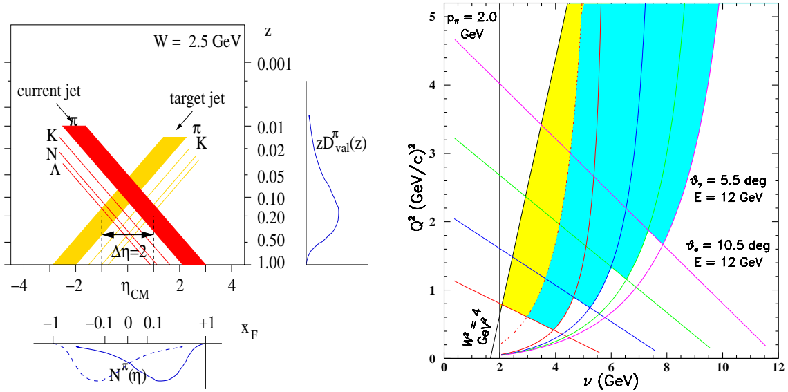
Figure 3.10: Left: Relation Between Elasticity z and Center-of-Mass Rapidity in semi-inclusive fragmentation for an invariant mass W of 2.5 GeV. Right: Kinematics plot for meson electroproduction experiments showing energy loss \nu versus momentum transfer squared Q^2 , assuming the HMS-SHMS magnetic spectrometer combination. Kinematics of interest are in the deep inelastic region, i.e. W^2 > 4 GeV 2 and accessible with HMS measuring the scattered electron (angle > 10.5^\circ ) and SHMS measuring the produced meson (angle > 5.5^\circ ). Beam energies of 6, 8, 10, and 12 GeV are assumed. The yellow area is what can be accessed at a 6-GeV beam energy with the present HMS-SOS magnetic spectrometer combination. The blue area is what can be accessed with the HMS-SHMS combination at a 12-GeV beam energy, and essentially corresponds to W > 2.5 GeV. For a fixed Q^2 , the large kinematic acceptance in \nu allows for a large variation in terms of elasticity z .
