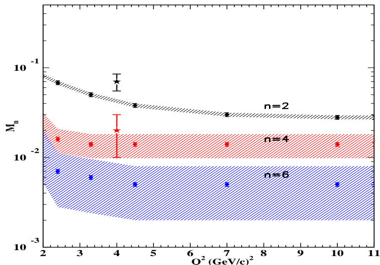
Figure 3.8: Lowest Moments of the Structure Function Differences \int_0^1 x^{n-2}(F_2^p - F_2^n)dx (left) and \int_0^1 x^{n-2}(g_1^p - g_1^n)dx (right), for n = 2 (black), 4 (red), and 6 (blue), as a function of Q^2 . Lattice QCD calculations (stars) are added at Q^2 = 4 (GeV/c) ^2 for n = 2 (black) and 4 (red). Experimental moments without including JLab data are indicated as hatched areas. The 12-GeV program will obtain precise moments for Q^2 \leq 10 (GeV/c) ^2 , for all polarized and unpolarized ( e, e' ) structure functions.
