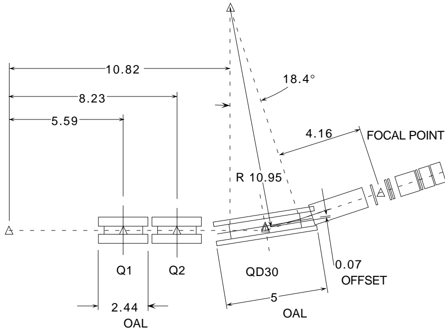
Figure 4.4: SHMS Spectrometer Key Dimensions (meters) showing the location of the two quadrupoles and the combined function magnet relative to the target and the detector stack.
