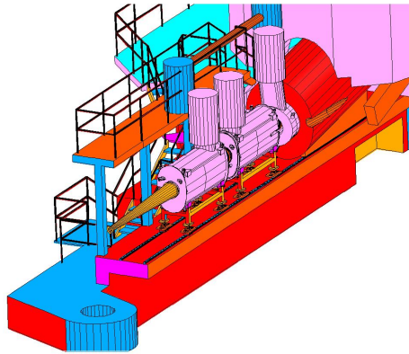
Figure 4.12: SHMS Pivot with Slider.
