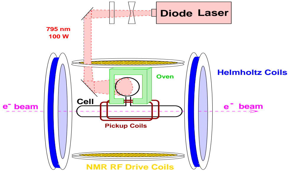
Figure 5.4: Schematic of the Spin-exchange Polarized ^3\text{He} Target. For clarity, only one set of Helmholtz coils is shown.
