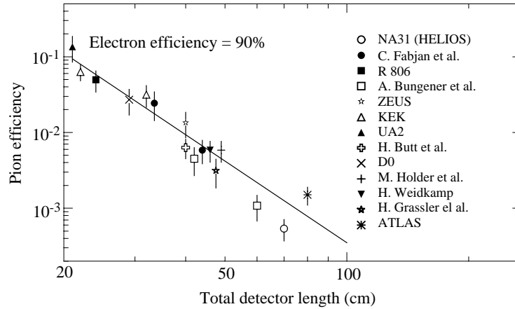
Figure 4.39: Pion Efficiency Measured (or Predicted) for different TRDs as a function of the detector length for an electron efficiency of 90%. (Figure from Ref. [37])
