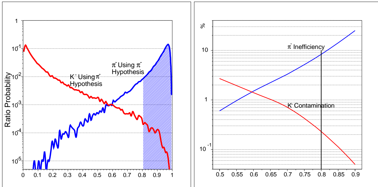
Figure 4.30: Pion/Kaon Discrimination using a Likelihood function applied to simulated energy loss distributions for 7-GeV/c particles in 12 wire chamber planes. For the (pion/kaon) hypothesis, only the eight (highest/lowest) measured energies are used. The left figure shows the distribution of pion likelihood ratios R = \frac{L_{\pi}}{L_{\pi} + L_K} when the incident particle is a kaon or a pion. On the right is shown the pion inefficiency and the kaon contamination as a function of the choice of cut, when equal numbers of pions and kaons are passed through the system.
