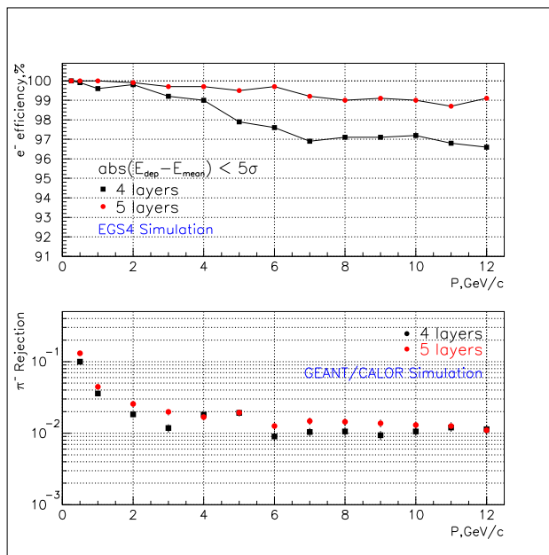
Figure 4.35: Electron detection efficiency (top panel) and pion rejection (bottom panel) obtained from the Monte Carlo simulation of the TF-1 Lead Glass Calorimeter. The calibration, coordinate correction and electronic effects are not included.
