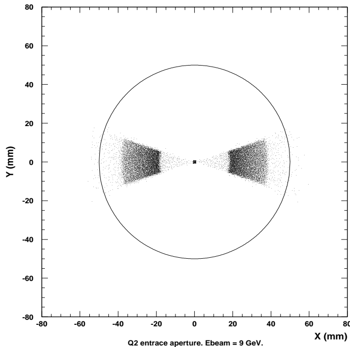
Figure 5.3: Scattered Electrons in the Møller Q2 Aperture for a Beam Energy of 9 GeV/c.
