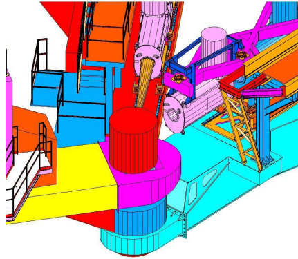
Figure 4.15: Hall C Pivot with (from left) SOS, SHMS, and HMS Attached.
