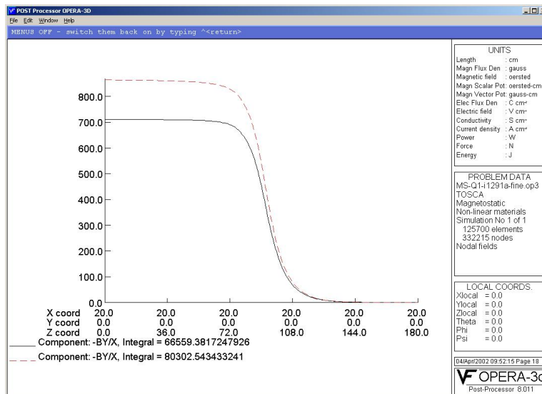
Figure 4.5: Q1 Gradient Comparison along Z.
