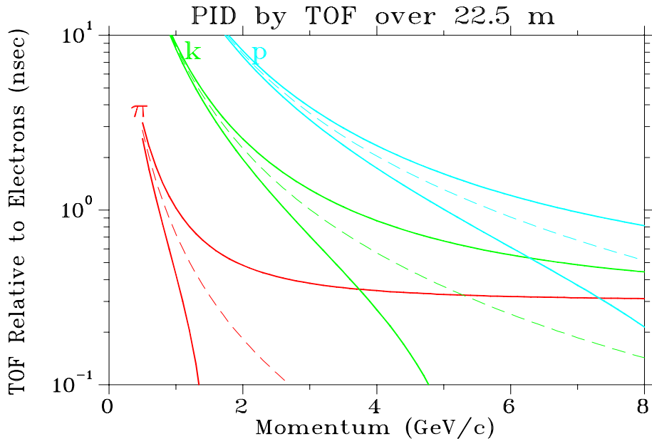
Figure 4.31: The dashed lines represent the time of flight (relative to electrons) versus momentum. The vase-shaped envelopes in solid lines demonstrate the limitations due to finite timing resolution ( \pm 1.5\sigma with \sigma = 200 ps assumed). At the points where the solid lines first intersect, the separation is only 3\sigma .
