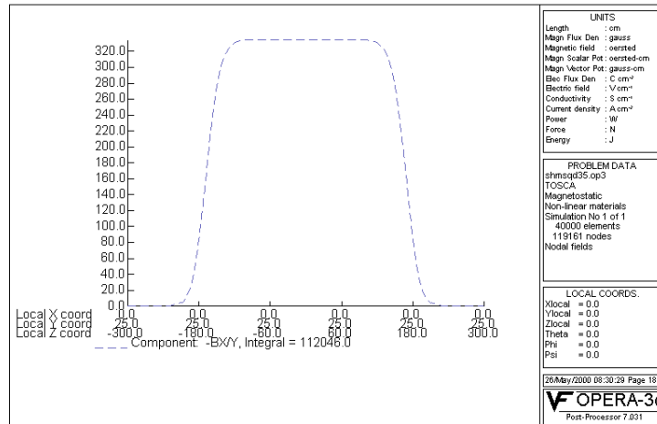
Figure 4.11: QD30 Integral B_x/y from -300 to 300 and gradient at (0,25,0)
