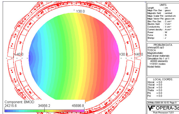
Figure 4.8: BMOD in QD30 Midplane (Gauss).
