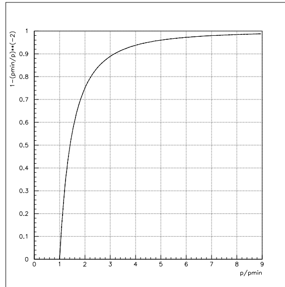
Figure 4.36: The Momentum Dependence of the Čerenkov Light Production Rate (eq.6)
