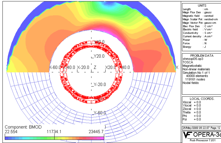
Figure 4.9: QD30 Yoke Saturation-Bmod (Gauss).
