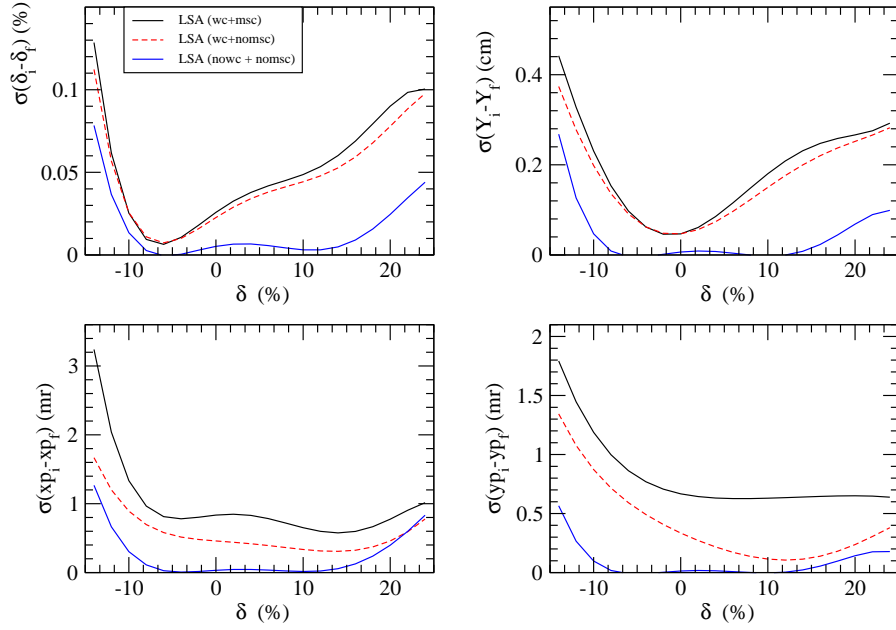
Figure 4.25: For the large solid angle (LSA) tune, plots of the resolutions in the target quantities \delta , Y_{tar} , y' and x' as a function of \delta for 7.5-GeV/c electrons. The solid black curve is the best estimate of real-world resolutions. The red dashed curve has only the effects of wire chambers resolutions and optics. The blue curve shows the limitation of the optical model. The subscripts f and i refer to the reconstructed and originally generated variables.
