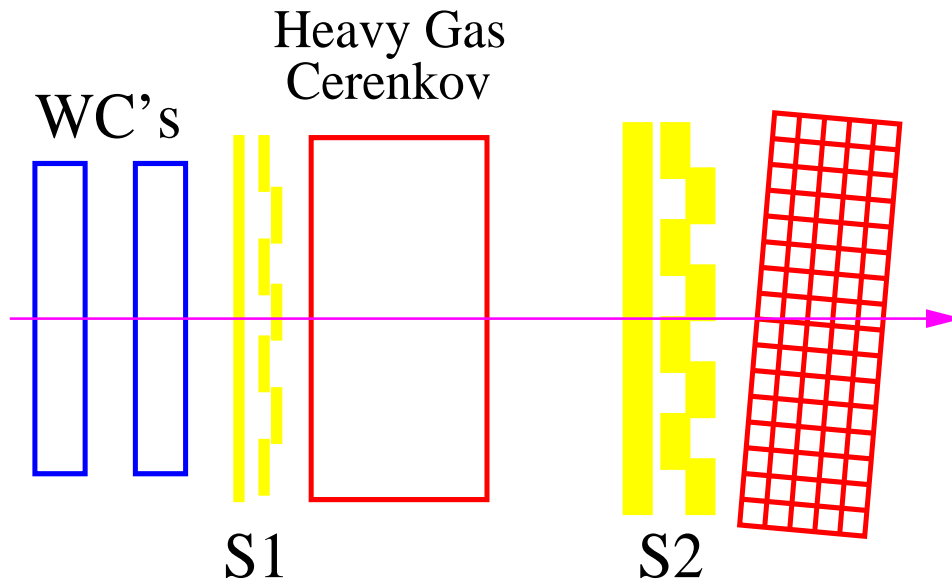
Figure 4.32: The thin S1 X and Y arrays will be located immediately after the wire chambers. The thicker S2 arrays will be located just before the electromagnetic calorimeter. (Drawing not to scale.)
