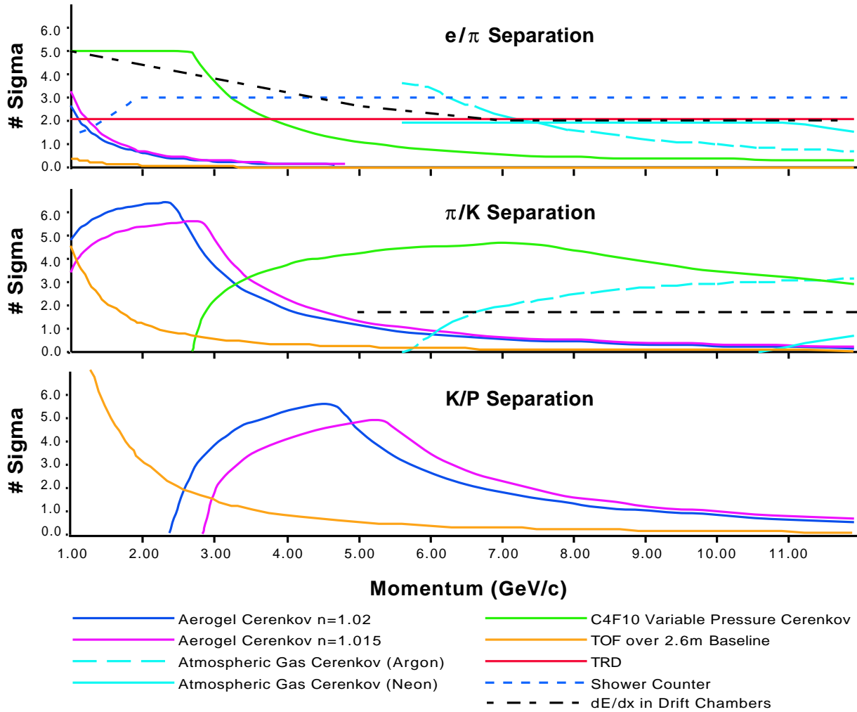
Figure 4.33: Particle Identification Resolving Power over the SHMS Momentum Range. The vertical scale in each graph is number of standard deviations which separate the two particle types shown, calculated for all of the relevant detectors in the system.
