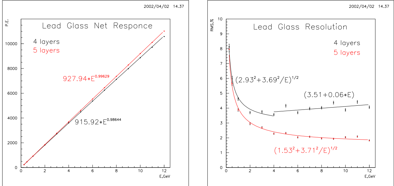
Figure 4.34: EGS4 Monte Carlo simulation of the linearity (left panel) and resolution (right panel) of a TF-1 Lead Glass modular calorimeter. The calibration, coordinate correction and electronic effects are not included.
