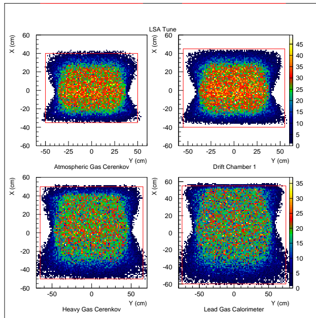
Figure 4.24: Plots of the vertical X versus the horizontal Y position at z=-60 cm ( Atmospheric Čerenkov ), z=-40 cm ( Drift Chamber 1 ), z=160 cm ( Heavy Gas Čerenkov ) and z=320 cm ( Lead Glass Calorimeter .) Spectrometer set for large solid angle tune with cuts of -15 < \delta < 25 % and -25 < Y_{tar} < 25 cm.
