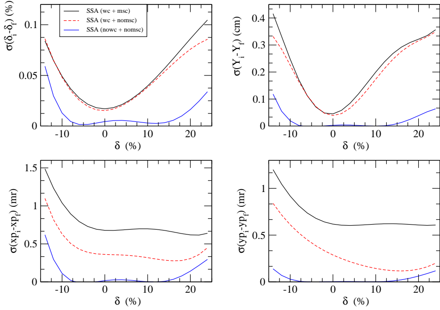
Figure 4.26: For the small solid angle (SSA) tune, plots of the resolutions in the target quantities \delta , Y_{tar} , y' and x' as a function of \delta for 7.5-GeV/c electrons. The solid black curve is the best estimate of real-world resolutions. Other curves explained in the text. The subscripts f and i refer to the reconstructed and originally generated variables.
