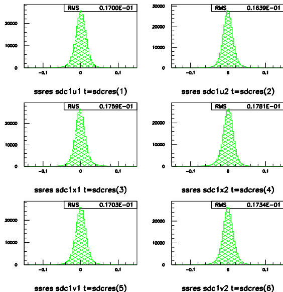
Figure 4.28: Measured Residual Distributions in the SOS Wire Chambers (cm).
