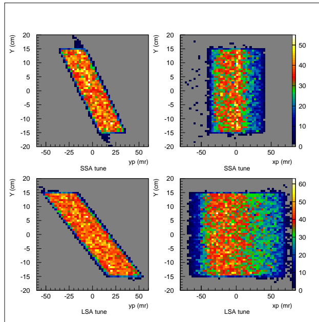
Figure 4.21: Y_{tar} Acceptance. Plots on the left are Y_{tar} versus y' and the plots on the right are Y_{tar} versus x' with cuts of -15 < \delta < 25 % and -25 < Y_{tar} < 25 cm. The top plots are with the small solid angle (SSA) tune and the bottom plots with the large solid angle (LSA) tune.
