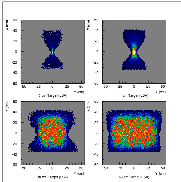
Figure 4.22: Plots of the Vertical X versus the Horizontal Y position at z=0 cm in the detector hut for target lengths of 0.5 cm, 4 cm, 30 cm and 50 cm. Spectrometer set for large solid angle tune with a cut of -15 < \delta < 25 %.
