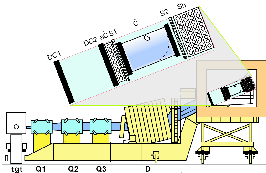
Figure 4.1: Sketch of the High Momentum Spectrometer showing the Magnets, the Carriage, and an expanded block diagram of the Detector Stack.
