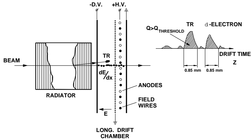
Figure 4.40: Single module with time expansion chamber (TEC) which includes a drift region and a proportional region. The output signals will consist of uniform dE/dx ionization with localized TR clusters and \delta -ray clusters.
