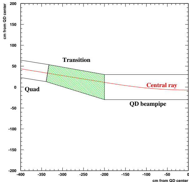
Figure 4.16: Track of the central ray from the exit of the last quad through the first half of the QD. The picture has been rotated so that the QD beam-pipe appears horizontal.
