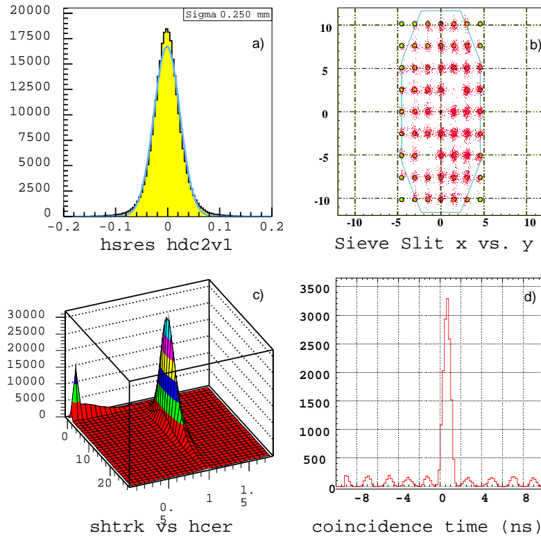
Figure 4.2: HMS Spectrometer Representative Data: Tracking capability is shown by a) Single-plane wire chamber resolution, and b) sieve slit reconstruction. Panel c) shows Shower Counter Energy vs. number of photons in the Čerenkov, demonstrating clear electron-hadron separation. Coincidence time resolution in the HMS-SOS hodoscope system is demonstrated in panel d) by the clear separation of particles from neighboring RF buckets.
