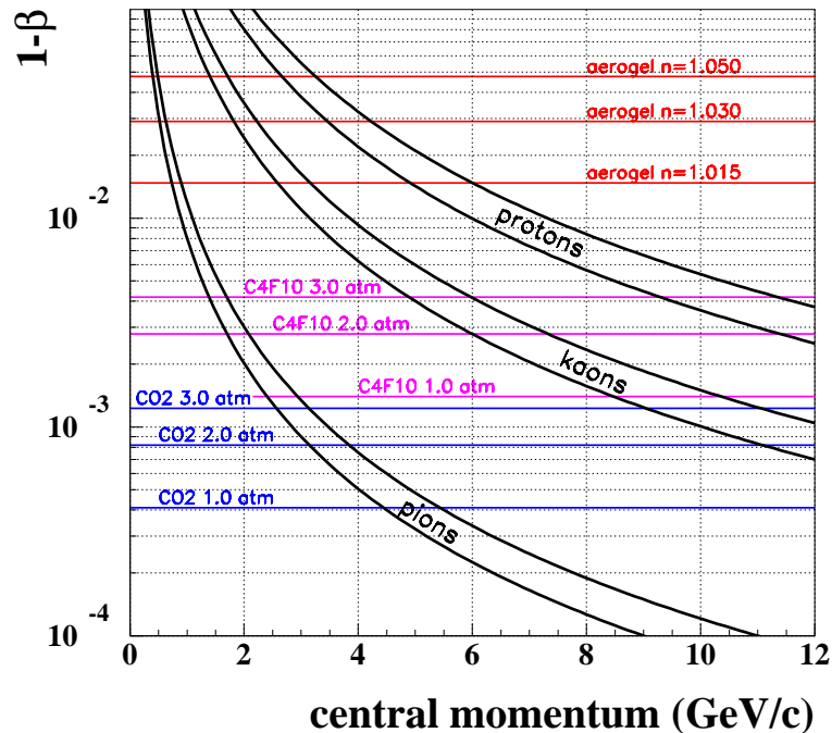
Figure 4.41: Hadron Velocity 1 - \beta as a Function of Momentum. For each particle a band is shown corresponding to a momentum acceptance of \pm 10\% . The horizontal lines show thresholds for different Čerenkov radiators.
