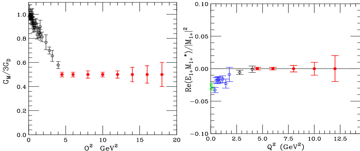
Figure 2.1: Left: The Magnetic Form Factor of the Nucleon-Delta Transition, scaled by the dipole form factor G_D = 1/(1 + Q^2/0.71) . Red circles are projected data using the HMS-SHMS magnetic spectrometer combination. Right: The ratio of electric quadrupole to magnetic dipole strengths for the excitation of the delta resonance. Green circles are photoexcitation data (Mainz and BNL), blue circles are JLab-CLAS data, black circles are JLab-Hall C data, and red circles show the projected range and uncertainties for JLab-Hall C.
