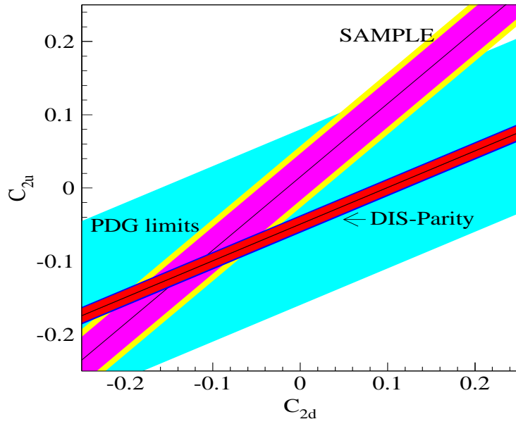
Figure 3.20: The Limits on C_{2u} and C_{2d} Listed by the Particle Data Group, SAMPLE, and the Proposed Experiment.
