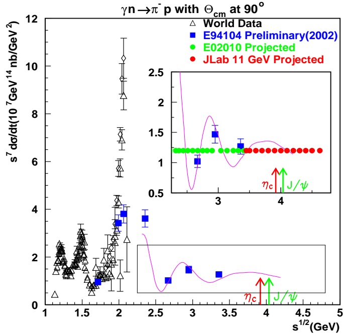
Figure 2.3: Projections for Measurements of the \gamma n \rightarrow \pi^- p Process at a Center-of-Mass Angle of 90^\circ . The HMS-SHMS combination is required to measure the high-momentum pion and proton. Open triangles are the existing world data. Blue squares are preliminary JLab data. The green (red) circles show the range possible with a 6-GeV (12-GeV) JLab beam energy. The purple oscillatory curve shows the anticipated effect of QCD oscillations. The arrows indicate the threshold of charm production.
