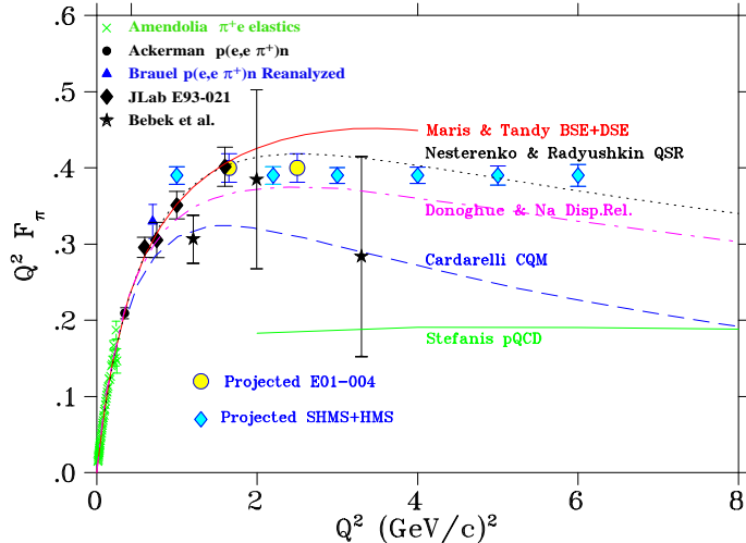
Figure 3.1: The \pi^+ Form Factor. Recent Hall C data are denoted by black diamonds. Blue diamonds denote 12-GeV projections. Other available data are shown as well. The curves are the results of theoretical calculations.
