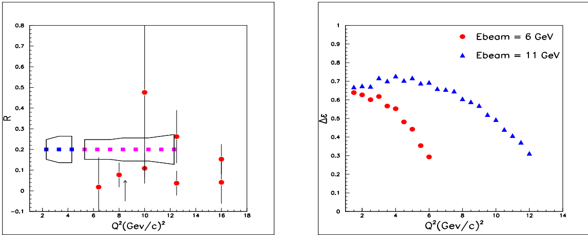
Figure 3.6: Left: projected measurements (blue for 6, pink for 11 GeV) at x = 0.8 for R , the longitudinal to transverse cross section ratio. The surrounding lines indicate the total uncertainty possible, as compared to the existing data set (red). The arrow corresponds to the Q^2 at which x = 0.8 corresponds to W^2 = 4 \text{ GeV}^2 . Right: The range in epsilon available for Rosenbluth separations at x = 0.8 as a function of Q^2 .
