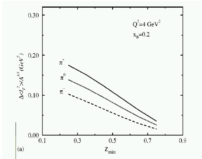
Figure 3.18: The Predicted Nuclear Transverse Momentum Broadening in Semi-Inclusive Pion Production.
