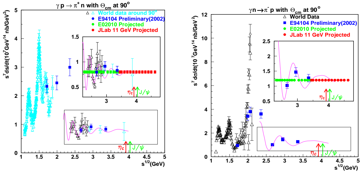
Figure 3.2: The Scaled Cross Section s^7 d\sigma/dt for the reactions p(\gamma, \pi^+)n (left) and n(\gamma, \pi^-)p (right) at \theta = 90^\circ , vs s . The existing data are shown in comparison to the 11-GeV projected data in the top inserts, and preliminary new data in the bottom inserts. Note that the new high energy data will straddle the c\bar{c} and J/\psi thresholds.
