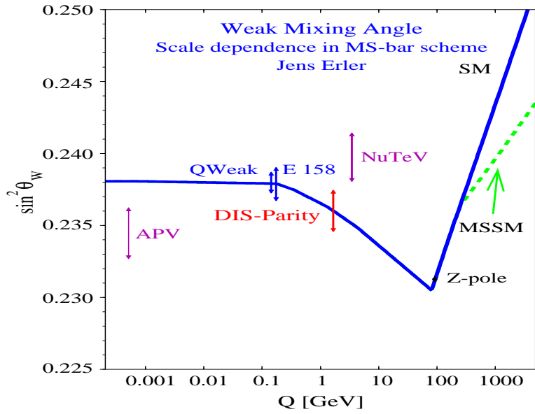
Figure 2.6: The Running of \sin^2 \theta_W Shown as a Function of Q . The proposed combined statistical and systematic precision of the deep inelastic scattering parity violation experiment at JLab (DIS-Parity) is shown in red. Also shown are the existing Atomic Parity Violation (APV) Cesium data and neutrino DIS (NuTeV) measurements, along with expected uncertainty of the approved JLab-QWeak and ongoing SLAC-E158 Møller experiments.
