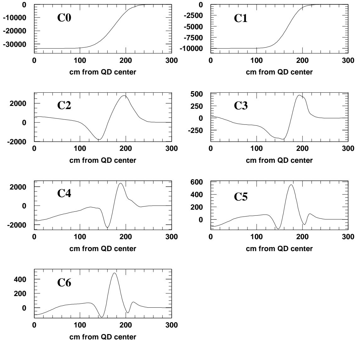
Figure 4.18: Polynomial Coefficients in the QD Magnetic Field Model as a function of z , the axial distance from the magnet center. (The functions are symmetric about z = 0 .) C0 is the dipole component, C1 the quadrupole component, and the others are higher order contributions. The vertical axes are the contribution to B_y at x = 30 cm, in gauss.
