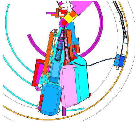
Figure 4.13: SHMS at 5 degrees. HMS at 10.5 degrees.
