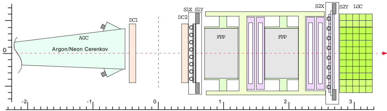
Figure 4.42: A Schematic of where the Focal Plane Polarimeter could fit into the SHMS Detector Package. There are two \text{CH}_2 analyzers, each followed by a set of drift chambers.
