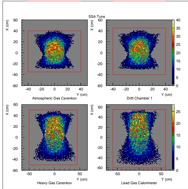
Figure 4.23: Plots of the vertical X versus the horizontal Y position at z=-60 cm ( Atmospheric Čerenkov ), z=-40 cm ( Drift Chamber 1 ), z=160 cm ( Heavy Gas Čerenkov ) and z=320 cm ( Lead Glass Calorimeter .) Spectrometer set for small solid angle tune with cuts of -15 < \delta < 25 % and -25 < Y_{tar} < 25 cm.
