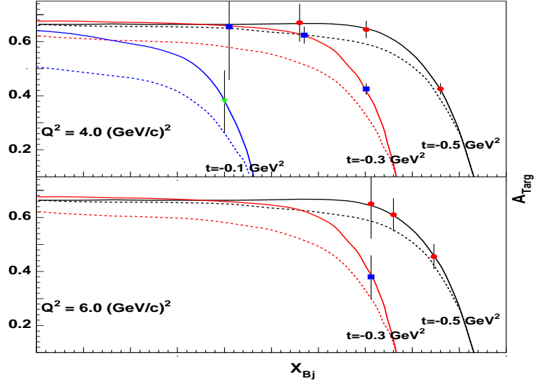
Figure 3.14: The Projected Results for Target Asymmetry in the Process en \rightarrow e'\pi^-p with a transversely polarized ^3\text{He} target. The solid and dashed lines are the calculations from Ref. [27] and represent different model assumptions regarding the GPDs.
