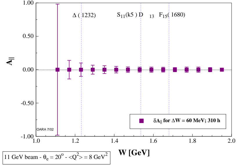
Figure 3.9: Expected Uncertainties for an 11-GeV Measurement of A_{||} in the \vec{H}(\vec{e}, e') reaction at Q^2 = 8 (\text{GeV}/c)^2 in the nucleon resonance region.
