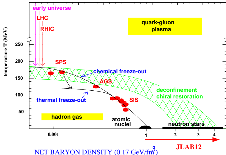
Figure 3.17: The Phase Diagram for Nuclear Matter.
