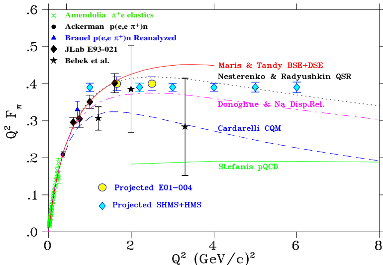
Figure 2.2: Projections for Measurements of the \pi^+ Elastic Form Factor with the HMS-SHMS Combination, ranging from confinement-dominated to perturbative-dominated quark-gluon dynamics. Green crosses denote results from elastic pion-atomic electron scattering. Recent Hall C data are denoted by filled diamonds. Blue diamonds denote 12-GeV projections. The curves represent model calculations of this transition.
