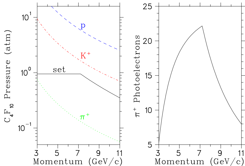
Figure 4.37: Left : Threshold \text{C}_4\text{F}_{10} pressure required for Čerenkov light generation from the particles indicated. The solid curve indicates the operating pressure planned for the detector. Right : Number of photoelectrons anticipated for the detector, taking into account the transmittance, reflectivity, and quantum efficiency functions of the detector components.
