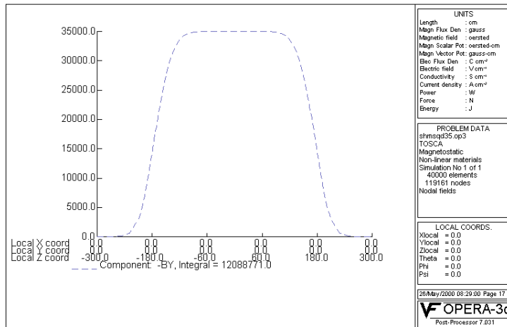
Figure 4.10: QD30 B_y and Integral from z = -300 to +300
