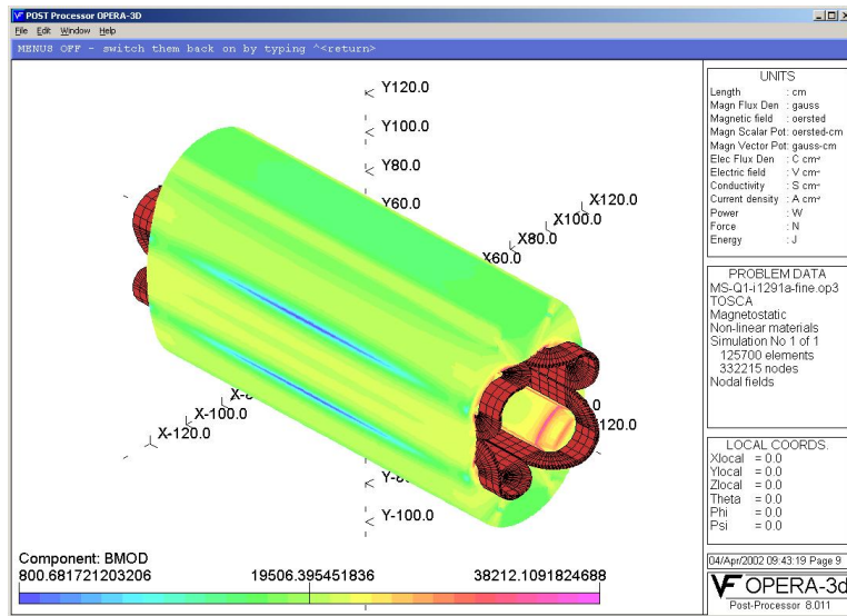
Figure 4.6: Magnetic Fields in Q1 at High Current.
