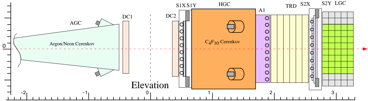
Figure 4.27: Block Diagram of SHMS Detector Arrangement.
