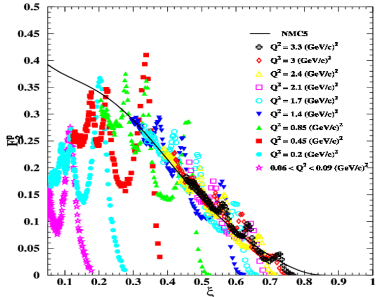
Figure 3.7: Duality Data from Hall C, depicting both the agreement in average strength and Q^2 dependence of the resonances and deep inelastic regimes for Q^2 > 0.8 ( \text{GeV}/c ) 2 , and the valence-like average shape of the lower Q^2 resonance data.
