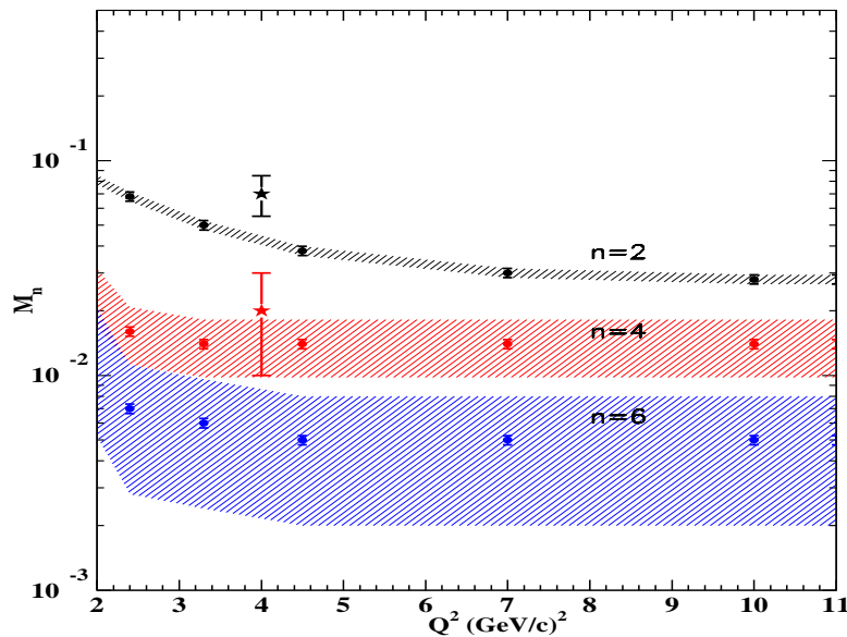
Figure 2.4: Lowest Moments of the Structure Function Difference \int_0^1 x^{n-2}(F_2^p - F_2^n)dx for n = 2 (black), 4 (red), and 6 (blue), as a function of Q^2 . Lattice QCD calculations (stars) are added at Q^2 = 4 \text{ (GeV/c)}^2 for n = 2 (black) and 4 (red). Experimental moments without including JLab data are indicated as hatched areas. The 12-GeV program will obtain precise moments for Q^2 \leq 10 \text{ (GeV/c)}^2 , for all polarized and unpolarized ( e, e' ) structure functions.
