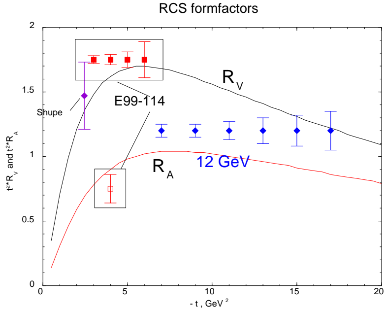
Figure 3.12: Projected measurements for wide angle Compton scattering as a function of -t , as compared to recent JLab data.
