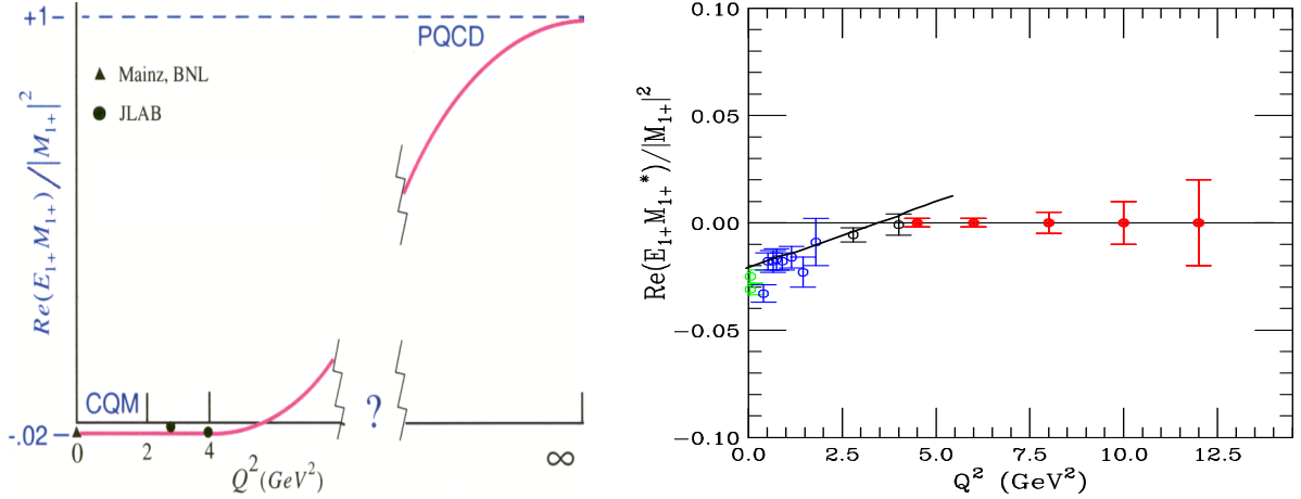
Figure 3.4: The Ratio of Electric Quadrupole to Magnetic Dipole Strength for the p \rightarrow \Delta transition. Left: The curve indicates the low Q^2 region of helicity non-conserving spin flip transition, consistent with the current data (points), as well as the unknown region where E_{1+}/M_{1+} \rightarrow 1 in the pQCD limit. Right: The same ratio, as measured (green from Mainz and BNL, blue from JLab CLAS, black from JLab Hall C), and as projected for JLab Hall C at 11 GeV (red). The curve comes from an analysis of the world’s unpolarized and polarized electroproduction data with the MAID dynamical isobar model [10, 11]. These authors state that the ratio shows a “clear tendency to cross zero, and becomes positive with increasing Q^2 . This is a possible indication of a very slow approach to the PQCD region.”
