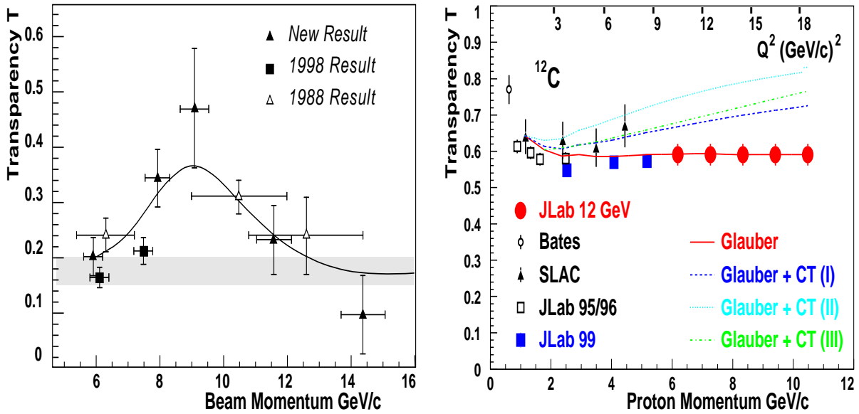
Figure 3.15: A(p,2p) Transparency Data from BNL (left), Compared to Recent and 11-GeV Projected Color Transparency Data from (e,e'p) measurements on Carbon in Hall C (right).
