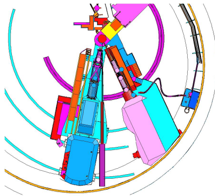
Figure 4.14: SHMS at 25 degrees. HMS at 10.5 degrees.
