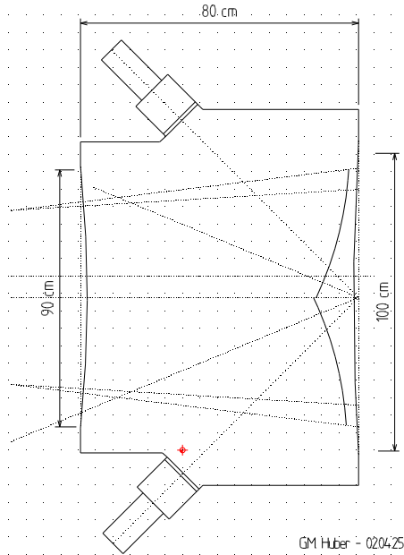
Figure 4.38: Schematic Design for the SHMS Heavy Gas Čerenkov Detector.
