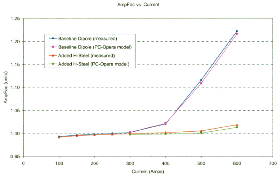
Figure 5.1: Renormalized Dipole Constant versus current for the existing “C” magnets (top two curves) and the reworked “H” magnets (bottom two curves). A momentum of 12 GeV/c corresponds roughly to 500A for “C” magnets. Saturation at 12 GeV/c in the “H” magnets will be less than 1%.
