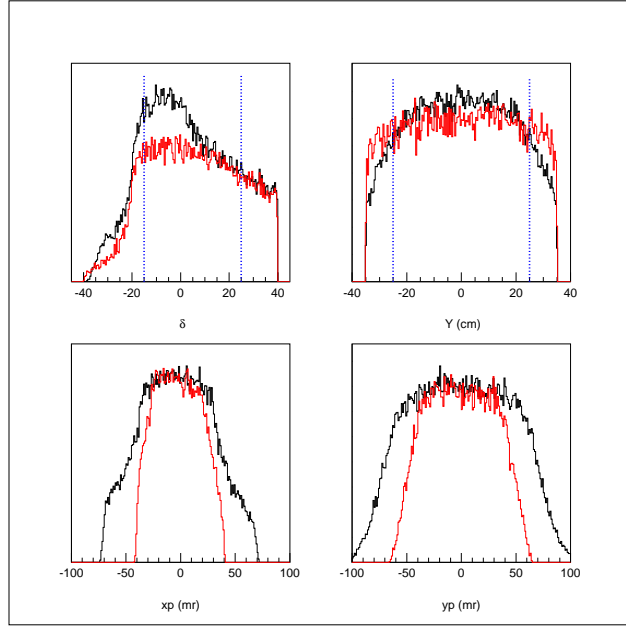
Figure 4.20: The Phase Space Acceptance plotted as function of \delta , Y_{tar} , y' and x' for the large solid angle (LSA) tune (black solid line) and the small solid angle (SSA) tune (red solid line). The y-axis is yield in arbitrary units and the LSA and SSA yields have been scaled to match each other at the maximum. The blue dotted lines indicate the limits of -15 < \delta < 25 % and -25 < Y_{tar} < 25 cm which were used in determining the detector size. The plots of y' and x' include the cuts of -15 < \delta < 25 % and -25 < Y_{tar} < 25 cm.
