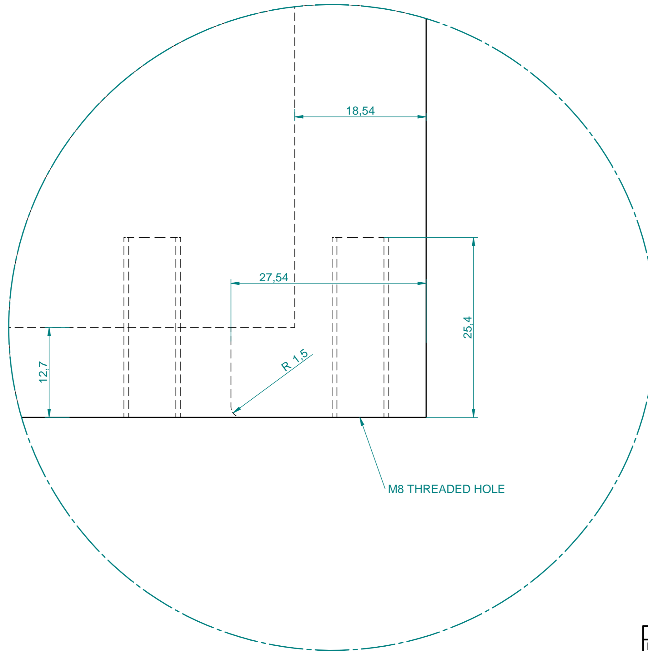
DETAIL A
