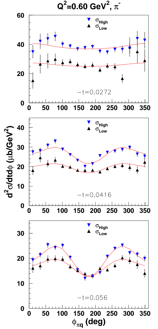
FIG. 9. (Color online) Unseparated experimental \pi^- cross sections as a function of azimuthal angle \phi at Q^2=0.60 GeV 2 , low \epsilon (black triangles) and high \epsilon (blue inverted triangles). The curves shown represent the fit of the measured values of the cross section to Eqn. 6. In this fit, all four parameters \sigma_{L,T,LT,TT} are extracted simultaneously, separate for each -t bin.
