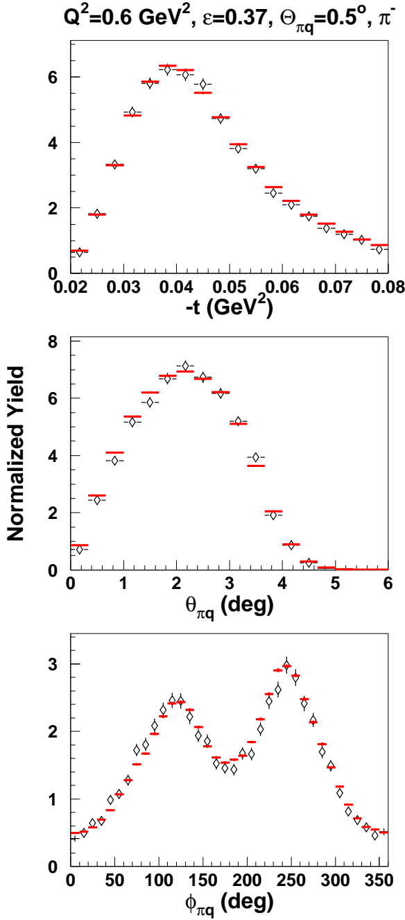
FIG. 8. (Color online) Normalized experimental \pi^- yield (black diamonds) in comparison to the quasi-free Monte Carlo simulation (red lines) for one HMS+SOS setting at Q^2=0.60 GeV 2 , low \epsilon .
