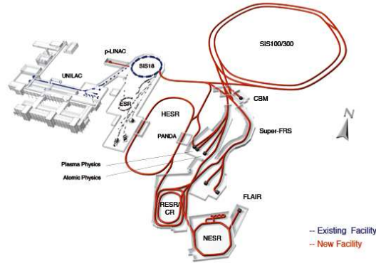
Figure 25: The Facility for Antiproton and Ion Research at GSI showing the exiting components and the planned new construction. The focus for hadron physics will be on research with precision, cooled, stored beams of antiprotons.
