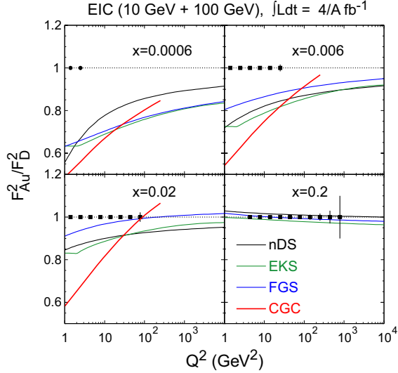
Figure 21: The ratio of the structure function F_2^{\text{Au}} in Au nuclei relative to the structure function F_2^{\text{D}} in deuterium nuclei as a function of Q^2 for several bins in x . The filled circles and error bars correspond respectively to the estimated kinematic reach in F_2 and the statistical uncertainties for a luminosity of 4/\text{A fb}^{-1} with the EIC. The curves labeled nDS, EKS and FGS correspond to different parameterizations of parton distributions at the initial scale for pQCD evolution, while the one labeled CGC corresponds to a Color Glass Condensate model prediction applicable at small x .
