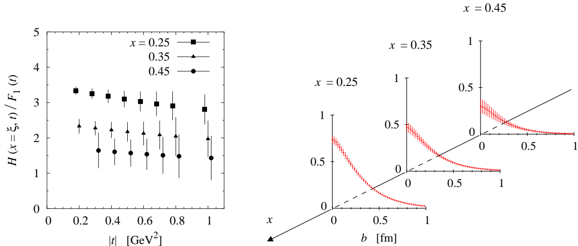
Figure 15: Spatial images of the proton from DVCS. Left : Projected JLab 12 GeV results for the Dirac GPD of the proton, H(x = \xi, t) , as a function of x and t , as extracted from the DVCS beam spin asymmetry, A_{LU} . Shown is the ratio of the GPD to the the proton’s Dirac form, F_1(t) . Right : Transverse spatial image of the proton obtained by Fourier–transforming the measured GPD [Di02]. The errors were estimated assuming a dipole–like t –dependence.
