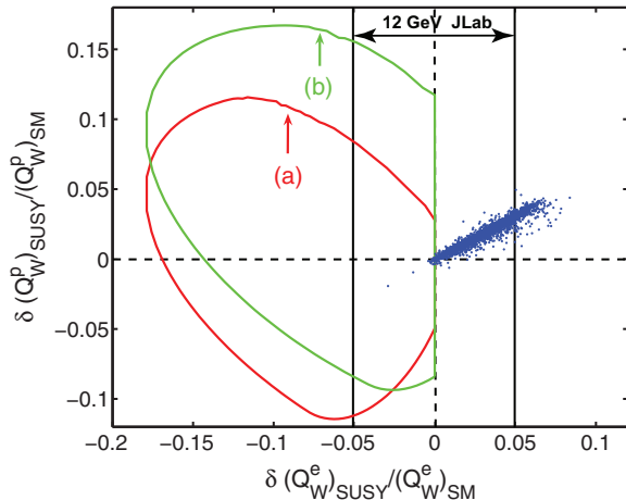
Figure 19: Relative shifts in Q_{\text{weak}}^e and Q_{\text{weak}}^p from SUSY effects (at 95% confidence level unless otherwise specified). The blue dots denote MSSM loop corrections for approximately 3000 SUSY-breaking parameter choices. The interior of the truncated elliptical regions (a) and (b) give possible shifts due to R-parity non-conserving SUSY interactions (95% confidence) using two different values of \delta|V_{ud}|^2/|V_{ud}|^2 [Ra06]. Because the lightest supersymmetric particle is unstable if R-parity is not conserved, these SUSY models offer no candidate for dark matter [Ku02]. The vertical bars illustrate what could be achieved by a 12 GeV Møller experiment at Jefferson Laboratory.
