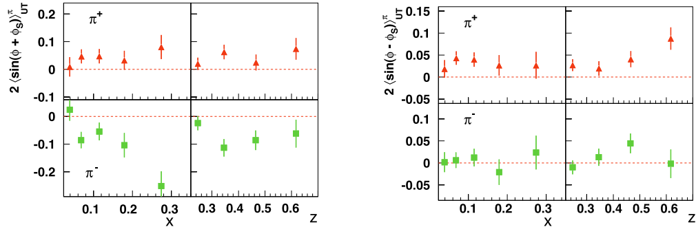
Figure 2: Collins and Sivers asymmetries measurements by HERMES[Ha06] for positive and negative pions.
