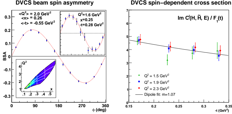
Figure 3: DVCS results from JLab with 6 GeV beam energy. Left : The beam spin asymmetry A_{LU} measured in the CLAS E01-113 experiment (preliminary), as a function of the azimuthal angle \phi . The main plot shows the data integrated over the entire kinematic range. The inlays show the kinematic coverage in x and Q^2 and the statistics achieved in a typical (x, Q^2, t) bin, illustrating the potential for fully differential measurements of DVCS observables with CLAS. Right : First measurement of the DVCS cross section by the Hall A experiment [Mu06, Ro06]. Shown is the dimensionless coefficient of the spin-dependent Bethe-Heitler/DVCS interference cross section at x = 0.36 as a function of t , for different values of Q^2 . The observed Q^2 -independence is consistent with the scaling behavior predicted by QCD. The coefficient is proportional to a linear combination of GPD's, which can be disentangled through target spin-dependent measurements.
