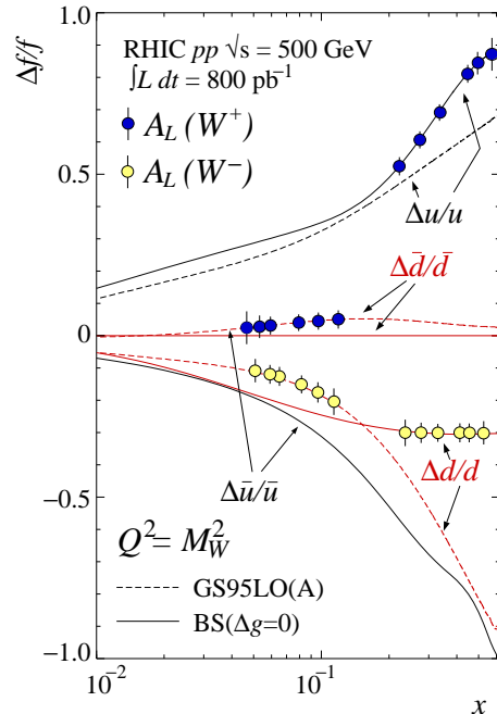
Figure 9: Expected asymmetries and error bars for W-boson production at polarized RHIC with center-of-mass energy 500 GeV. They are sensitive to polarized quark and antiquark distributions
