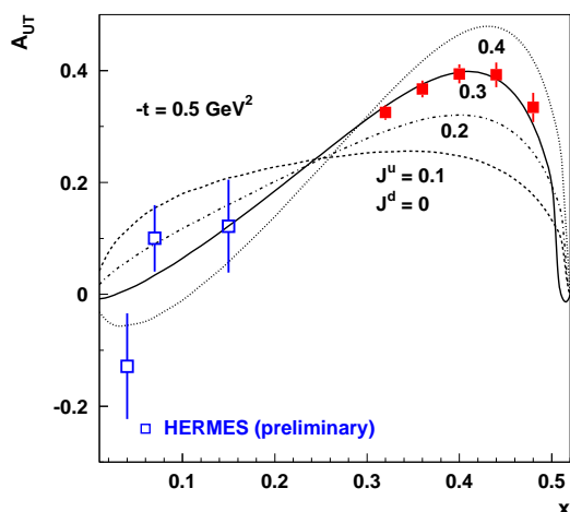
Figure 16: Sensitivity of the transverse target spin asymmetry in deeply-virtual \rho^0 production to the total u -quark angular momentum in the proton, J^u . The curves represent a theoretical prediction based on GPD models in which J^u appears as a free parameter [Go01]. The red data points illustrate the precision of the projected measurements at 12 GeV.
