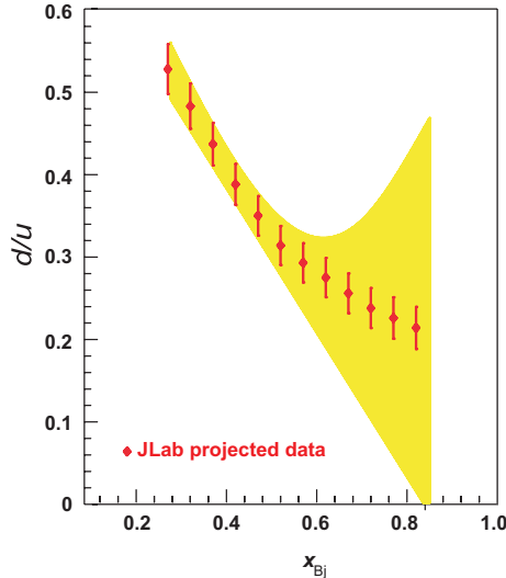
Figure 12: Projected measurement of the ratio of d - and u -quark momentum distributions, d(x)/u(x) , at large x , made possible by the 12 GeV Upgrade. The shaded band represents the uncertainty in existing measurements arising from nuclear Fermi motion effects.
