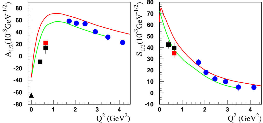
Figure 7: The extracted \gamma N \rightarrow N^*(1440) transverse (left panel) and scalar (right panel) form factors compared with the results from relativistic quark model calculations (Ref. [Ca95], red curves, and Ref. [Az07], green curves).
