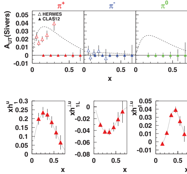
Figure 13: Projected transverse spin asymmetry from the Sivers effects ( A_{UT}^{\sin(\phi-\phi_S)} ) in single \pi production with CLAS at 11 GeV (top) and transverse spin distributions extracted from transversely polarized, longitudinally polarized and unpolarized target measurements (bottom). Curves are predictions for transversity, h_1 , [An07], Mulders, h_{1L}^\perp [Ef05] and Boer-Mulders, h_1^\perp , distributions [Ba04] for u -quarks.
