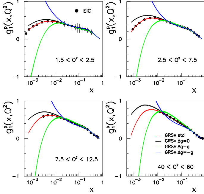
Figure 22: Projected EIC data for the proton structure function g_1(x, Q^2) as a function of x in four Q^2 bins, for 7 GeV electrons colliding with 150 GeV protons at an integrated luminosity of 5 \text{ fb}^{-1} . The curves show theoretical predictions based on different sets of spin-dependent parton distribution functions that mostly differ in the gluon helicity distribution.
