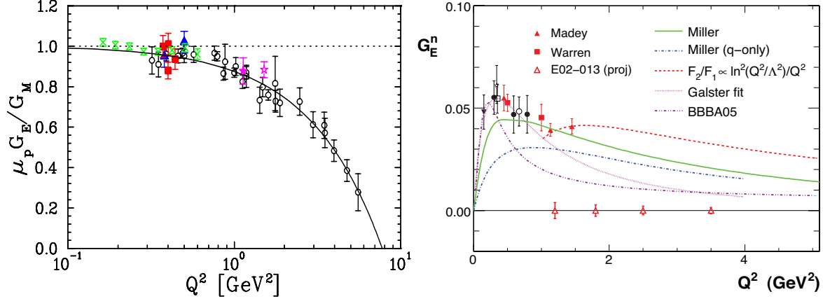
Figure 4: a): recent results from polarisation measurements of \mu_p G_E^p / G_M^p from Ref. [Ar06]. The solid line is a linear fit to the JLab data, \mu_p G_E^p / G_M^p = 1 - 0.13(Q^2 - 0.04) . b): Collection of G_E^n data compared to calculations and the Galster parametrisation [Ga71]. Projected sensitivities of a recently completed JLab Hall A measurement are also shown.
