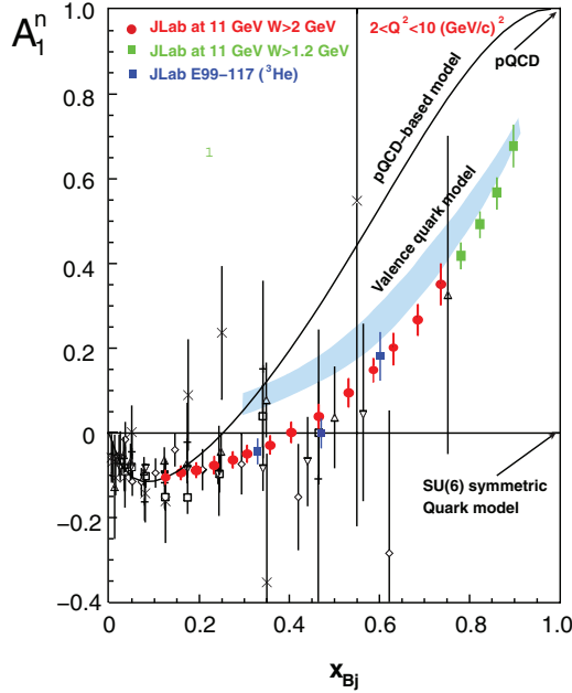
Figure 11: Projected measurement of the neutron polarization asymmetry, A_1^n , with the 12 GeV Upgrade. The shaded band represents the range of predictions of valence quark models; the solid line is the prediction of a pQCD-based quark model.
