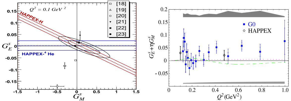
Figure 5: a): 68 and 95% C.L. constraints in the G_E^s - G_M^s plane from recent HAPPEX data [Ac07]. Various theoretical predictions are also shown. b): the combination G_E^s + \eta G_M^s as a function of Q^2 from the G0 experiment [Ar05a]
