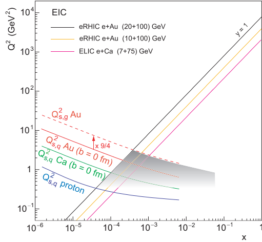
Figure 20: Kinematic acceptance and exposure of the predicted gluon saturation regime in the (x, Q^2) plane for the EIC. The accessible regions fall to the right of the three diagonal straight lines, representing different choices for beam energies (per nucleon in the case of ion beams) and maximum mass of the ion beams. Curves showing the quark saturation scale Q_s^2 for protons, Ca, and Au nuclei are superposed on the kinematic acceptance. As indicated, the gluon saturation scale in Au nuclei is larger by the color factor 9/4 . The shaded area indicates the kinematically accessible region of saturated gluon density that should be reached in the maximum-energy e+Au collisions considered.
