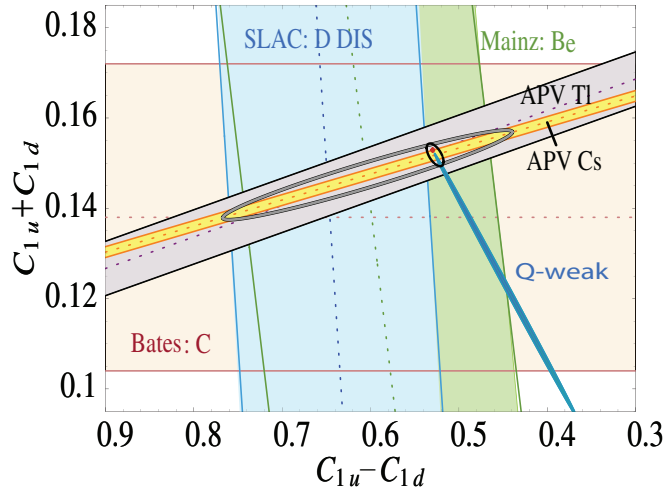
Figure 8: The anticipated knowledge of the weak charges associated with an axial coupling to the electron and a vector coupling to the up and down quarks after the Q_{Weak} measurement. The large grey contour displays the previous experimental limits (95% confidence level, CL) reported by the Particle Data Group, together with the prediction of the Standard Model (small red dot). The solid teal ellipse denotes the anticipated constraint provided by the upcoming Q-weak measurement on the proton, (at 1 standard deviation) while the small black contour (95% CL) indicates the full constraint obtained by combining all results. All other experimental limits shown are displayed at 1 standard deviation [Yo07].
