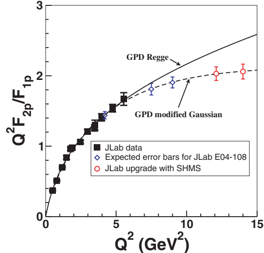
Figure 10: The JLab 6 GeV data on the ratio of proton form factors, F_2^p/F_1^p , and the projected measurements at 12 GeV. Perturbative QCD implies that F_2^p/F_1^p \sim 1/Q^2 for Q^2 \rightarrow \infty . The graph illustrates the potential of form factor measurements at 12 GeV to discriminate between GPD models. Shown are the predictions of a Regge-based GPD model [Gu04] and a model based on soft Gaussian nucleon wavefunctions modified by a short-range interaction [St03d].
