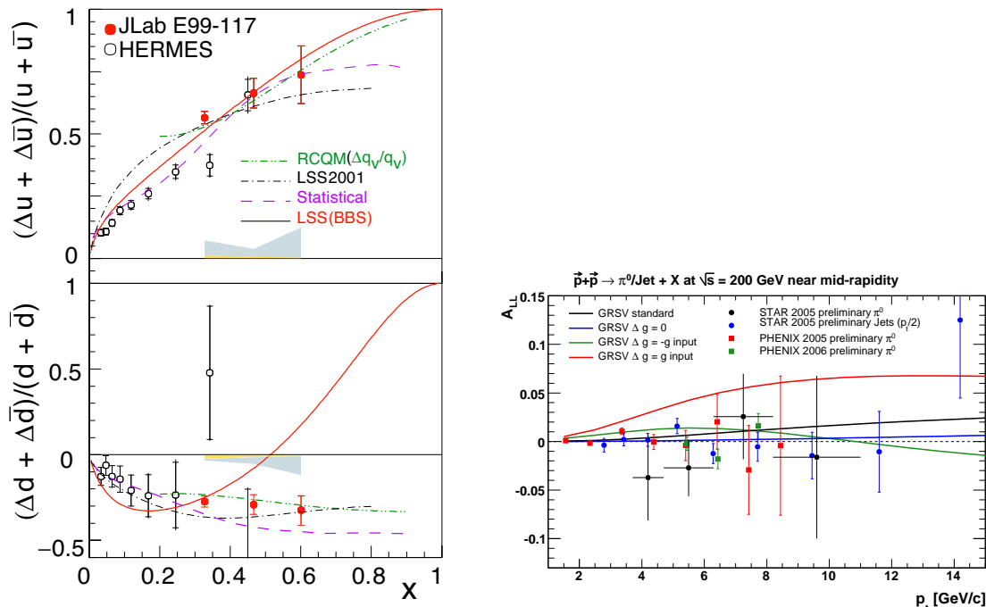
Figure 1: (a) Left: JLab (6 GeV) results for polarized quark distributions derived from the neutron virtual photon asymmetry A_1^n . The LSS(BBS) curves are pQCD predictions assuming hadron helicity conservation. (b) Right: PHENIX and STAR preliminary data on double spin asymmetry in inclusive \pi^0 and jet production at RHIC, respectively, at \sqrt{s} = 200 GeV. Also shown are theoretical curves which were pQCD fit to the deep inelastic fixed-target data or some models inspired with additional assumptions of polarized gluon distribution [G196]
