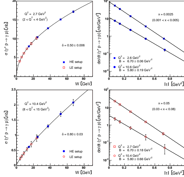
Figure 23: Left: projected results for total DVCS cross section measurements with an EIC, as a function of invariant \gamma^*p mass W , for two values of Q^2 . Right: t differential DVCS cross section for two representative values of x and Q^2 . The projections assume a high-energy setup (10 GeV on 250 GeV), with an integrated luminosity of 530 \text{ pb}^{-1} for the smaller x -value, and a low-energy setup (5 GeV on 50 GeV) with 180 \text{ pb}^{-1} for the larger x -value. The estimates of the event rates here assume 100% detector acceptance.
