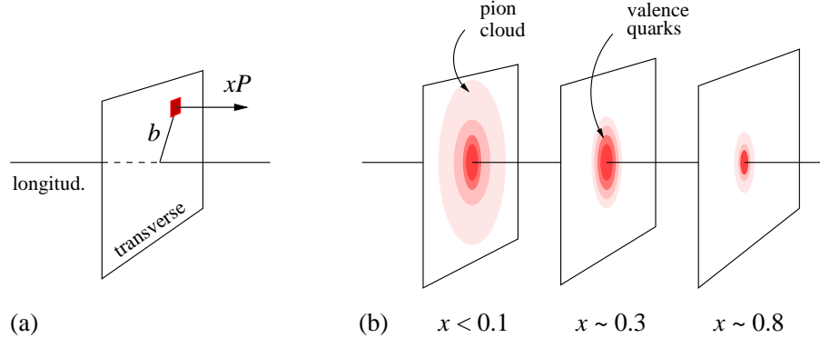
Figure 14: Nucleon tomography. (a) The Fourier transform of the GPD describes the transverse spatial distribution of quarks with longitudinal momentum fraction x . (b) It produces a set of 2-dimensional “tomographic” quark images of the nucleon [Bu03], which e.g. allow one to identify the valence quark core ( x \geq 0.3, b \ll 1 fm) and the pion cloud ( x \leq 0.1, b \sim 1 fm) [St03a].
