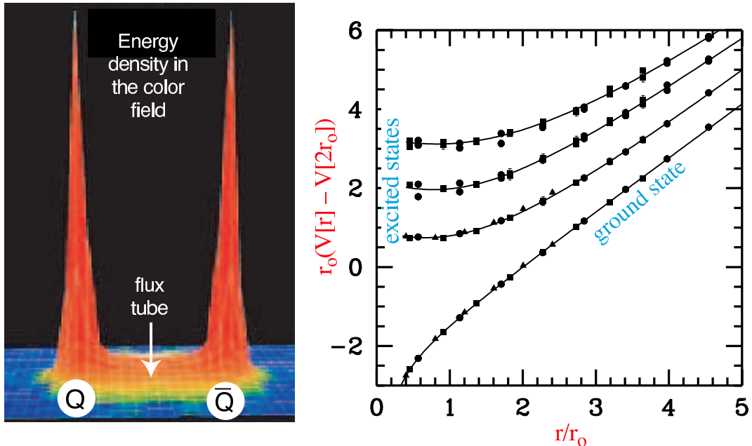
Figure 6: (left) A lattice QCD calculation of the action density in the color field between a quark and an anti-quark. The density peaks at the positions of the quarks and is confined to a tube between the quarks. This calculation is for heavy quarks in the quenched approximation. (right) The corresponding potential between the quarks. The ground state potential has a 1/r dependence at small distances and is linear for large distances.
