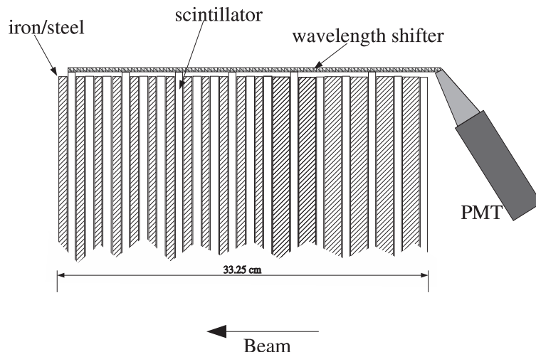
Figure 220: Sketch of an upstream photon veto segment. The 18 scintillator layers are arranged into three alternating orientations: x , u , and v . Shown is the light collection for one such orientation. The light collecting ends of the scintillators are joined together via a wavelength shifter which is oriented perpendicular to the scintillators. The wavelength shifter is used to redirect the light through 90^\circ and out the upstream end of the solenoid to photomultiplier tubes (PMT).
