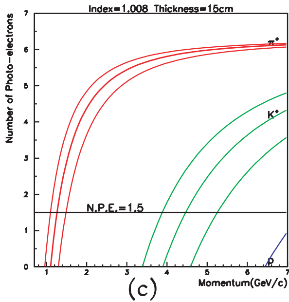
Figure 151: (a) The deviation of velocity from 1 vs. momentum for protons, pions and kaons. Dotted lines indicate the momentum bite of the spectrometer. (b) A1 performance with index of 1.015 and thickness of 9 cm. (c) Estimated number of photo-electrons vs. momentum for index of 1.008 and thickness of 15 cm. (d) Estimated number of photo-electrons vs. momentum for index of 1.030 and thickness of 10 cm.
