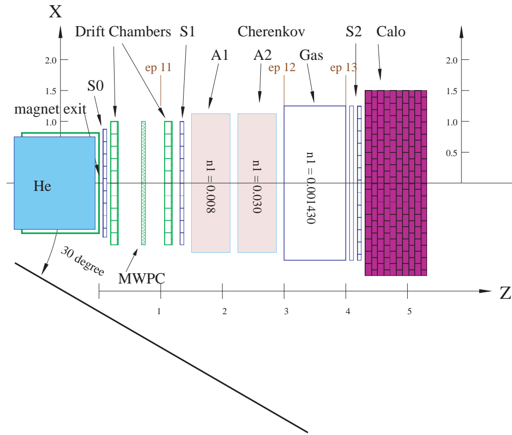
Figure 149: Configuration of the detector package for electrons (top) and hadrons (bottom).
