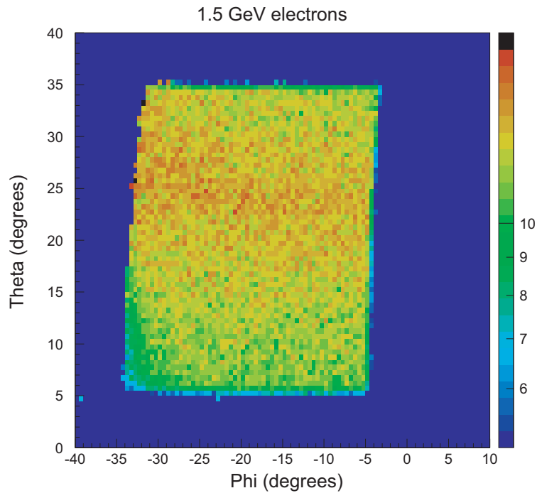
Figure 167: Left: Distribution of the number of photoelectrons N_{pe} for the HTCC in the \phi - \theta plane. The simulation was done for electrons of 1.5 GeV/c momentum. The solenoidal field was included in the simulation at full strength of 5 Tesla central field. The phi motion of the electrons in the solenoid field leads to a slight broadening of the photon distribution at the Winston cones and PMTs. Right: Average N_{pe} versus the polar angle (projection of the graph on the left onto the \theta axis). The \theta -dependence in N_{pe} is due to the different radiator gas length for different polar angles.
