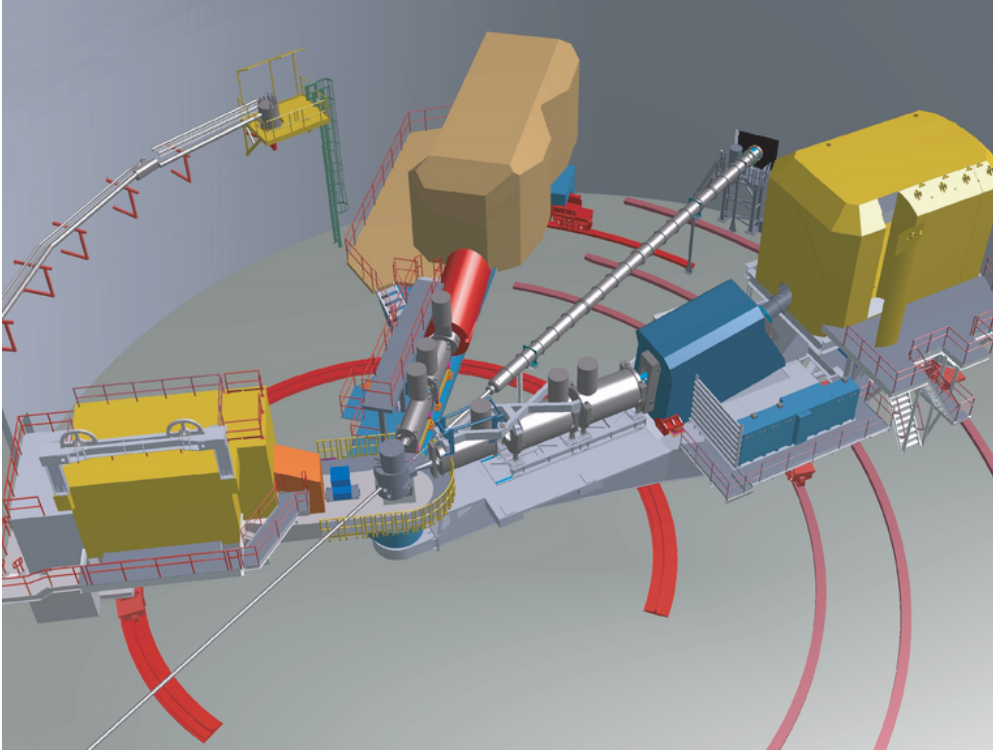
Figure 26: A CAD drawing of the new SHMS spectrometer installed in Hall C together with the existing HMS and SOS spectrometers.
