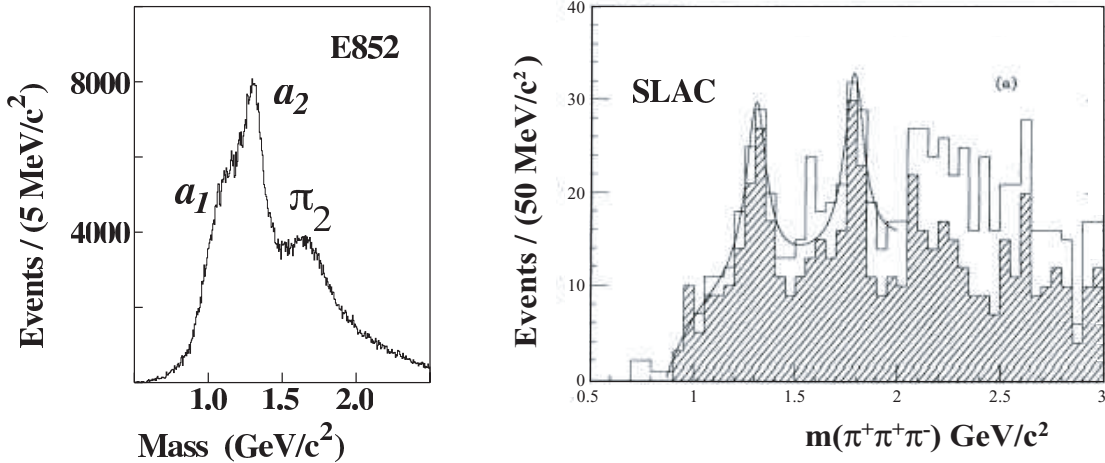
Figure 38: (left) The 3\pi mass spectrum from the reaction \pi^-p \rightarrow \pi^+\pi^-\pi^-p at 18 GeV/c from E852 at Brookhaven. (right) The 3\pi mass spectrum from the reaction \gamma p \rightarrow \pi^+\pi^+\pi^-n at 19 GeV from SLAC. The shaded area identifies the portion of the 3\pi spectrum that included a \rho meson.
