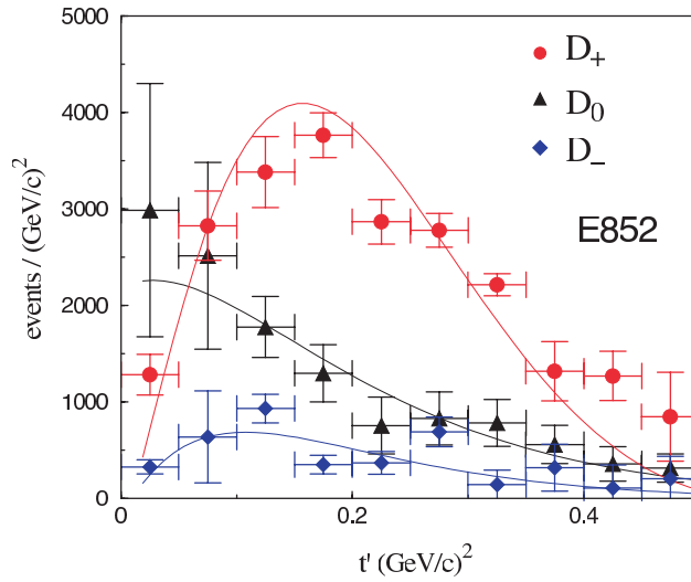
Figure 40: The distribution in |t'| where t' = t - t_{min} for the D -waves after a PWA of the \eta\pi^0 system from the reaction \pi^-p \rightarrow \eta\pi^0n at 18 GeV/c. The curves are fits to expected Regge exchanges for the various D -waves.
