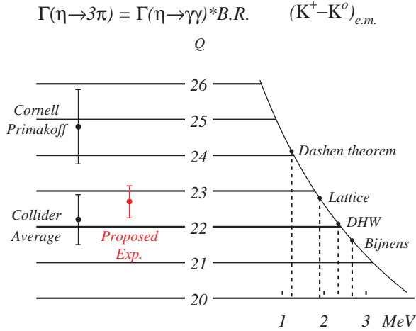
Figure 21: The importance of \Gamma_{\eta\rightarrow\gamma\gamma} in the measurement of the quark mass ratio \mathcal{Q} , where \mathcal{Q}^2 = \frac{m_s^2 - \hat{m}^2}{m_d^2 - m_u^2} and \hat{m} = (m_u + m_d)/2 . The l.h.s. indicates the values of \mathcal{Q} corresponding to the Primakoff and collider experimental results for \Gamma_{\eta\rightarrow\gamma\gamma} , and the projected result for Jefferson Laboratory with 12 GeV. The r.h.s. shows the results for \mathcal{Q} obtained with four different theoretical estimates of the electromagnetic self energies of the kaons. The figure is adapted from Leutwyler.
