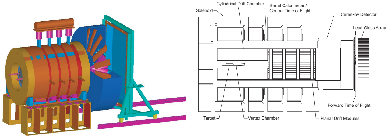
Figure 216: A 3D cutaway view of the GLUEX detector (left) and schematic diagram of its major subsystems (right)
