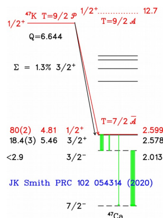
Figure 20-1: ^{47}_{20}\text{Ca}^{27} 's single 1/2^+ state contains most of the A config.
